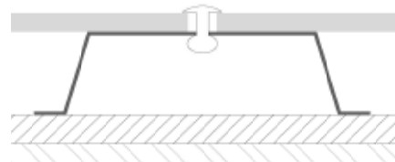
Installation of sliding points [no fixation ring]
