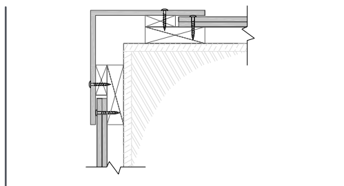
Outside corner with corner element
